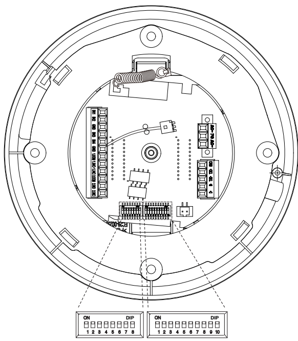
Camera ID DIP Switch (SW1) Communication Protocol DIP Switch(SW2)
